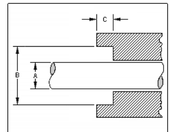
Seal Cavity With No Retainer
