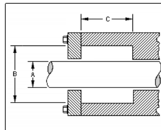
Seal Cavity With Retainer
