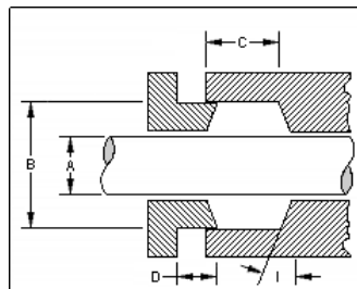
Stuffing Box
