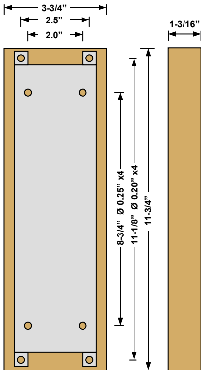
HAB311, HAB311B back and side view
